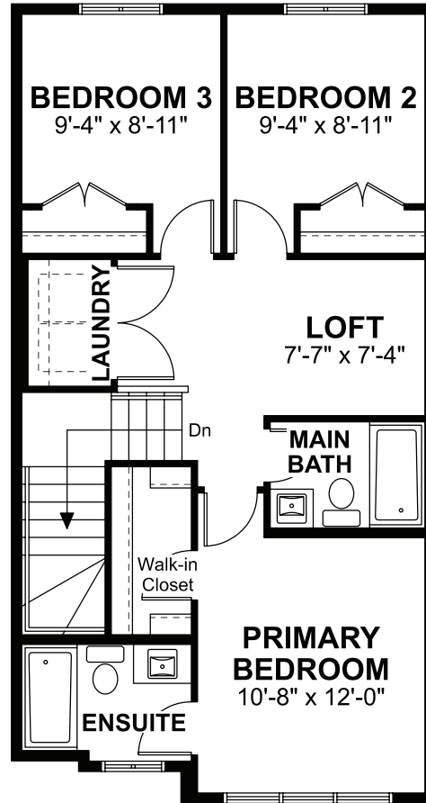
Optional Alternate Upper Level
