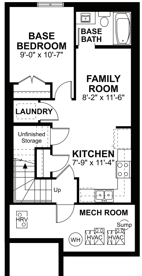
Optional Lower Level Legal Suite
